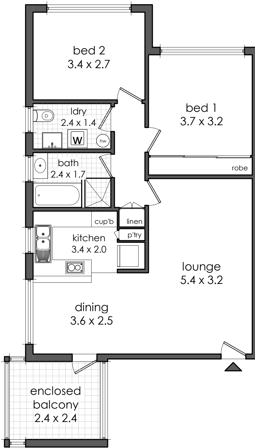
floor plan
