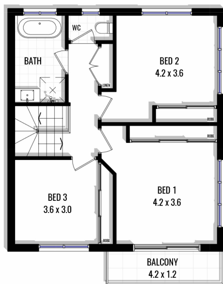
FIRST LEVEL
